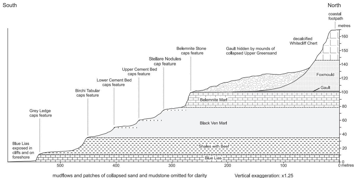
Figure 1. Simplified geological section through the central part of the Black Ven landslip showing the relationship of the topography to thin beds of limestone within the Charmouth Mudstone Formation.
