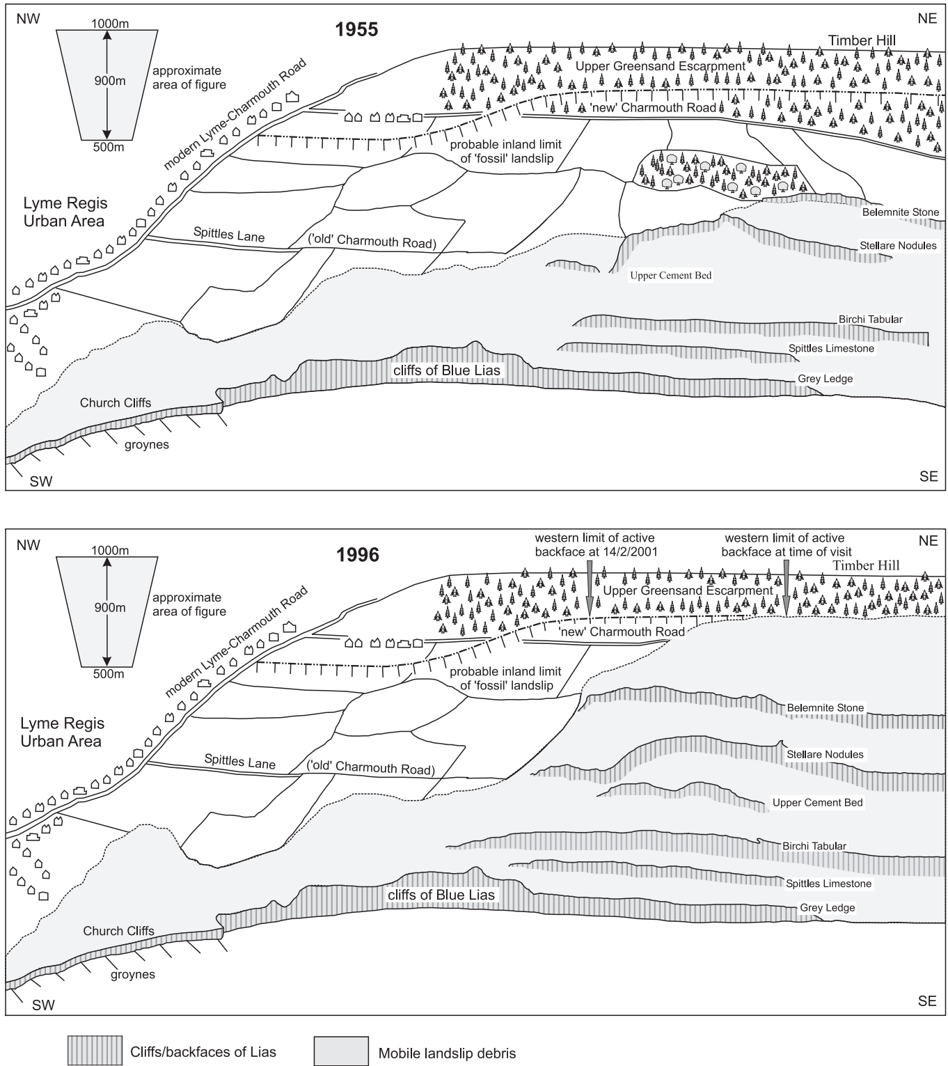
Figure 2. Sketch diagrams of the western part of the Black Ven-Spittles 'fossil' landslide showing the reactivation between 1955 and 1996. Based on oblique air photographs; uncorrected for parallax.
