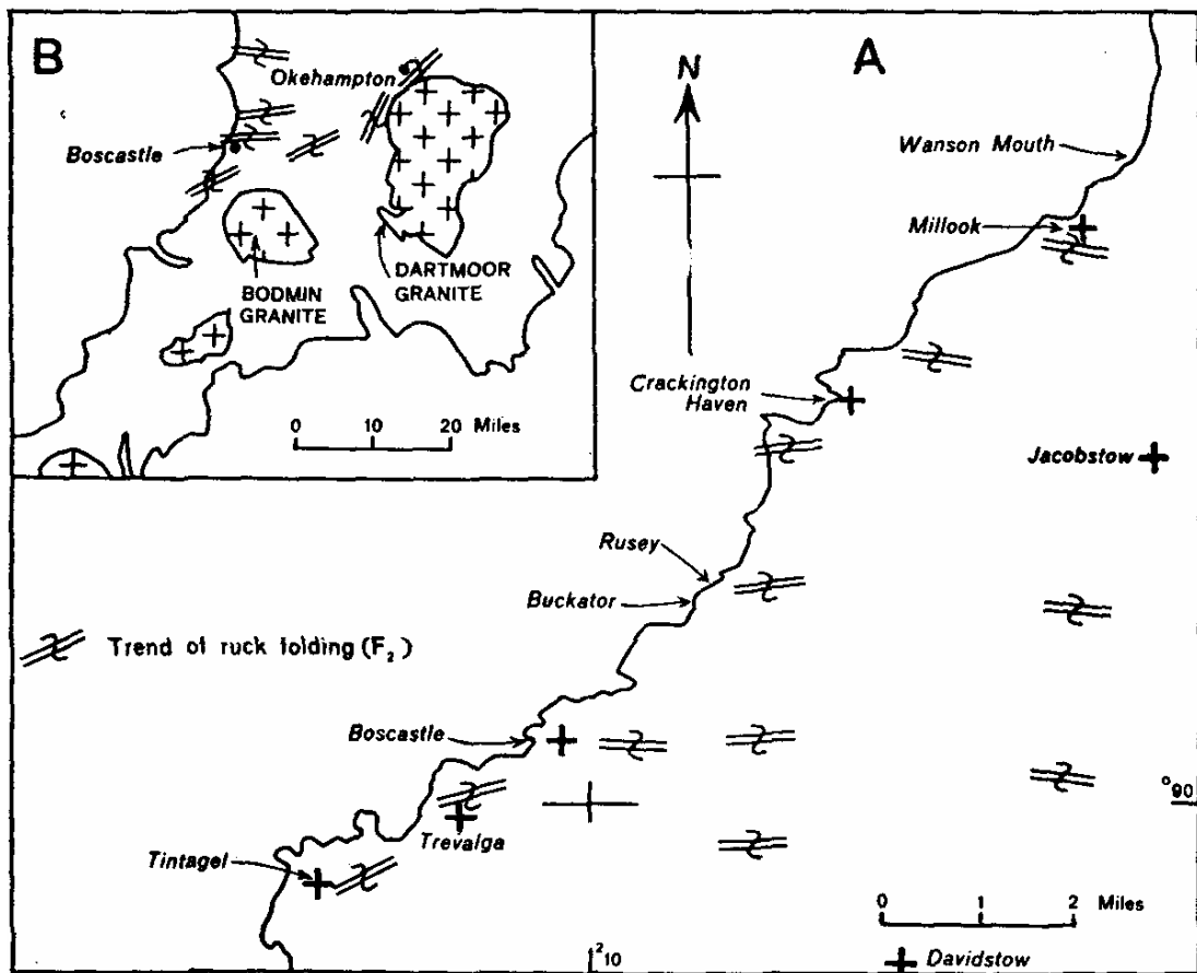
FIGURE 1. A, Sketch-map showing trends of late ruck-fold axes (F2) in the Boscastle area. (Data for Tintagel area supplied by Mr. M. C. McKeown.) B, Sketch-map showing trends of late ruck-fold axes (F2) in the area to the north of the Bodmin-Dartmoor granite. The fold trends in the Okehampton area are from Dearman (1959 and 1964). The outline map of Devon and Cornwall is corrected for the effects of Tertiary faulting after Dearman (1963).
