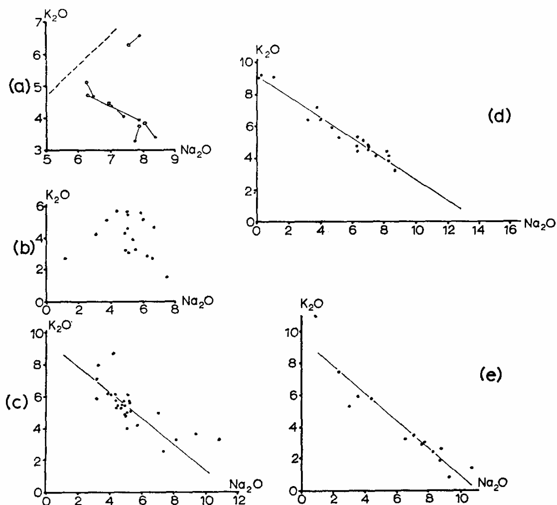
FIGURE 2. \text{Na}_2\text{O} - \text{K}_2\text{O} variation diagrams (molecular quotients x 100). (a) Pitchstones. Dots---rock; circles=glass. Dashed line = alkali ratio of the ternary minimum at 500 bars \text{PH}_2\text{O} . (b) Type I granites, Dartmoor. (c) Types 2, 3 and 4 granites, Dartmoor. Regression equation, Y = -0.82 X + 11.6 , r = -0.92 . (d) Tregonning-Godolphin granites. Regression equation, Y = -0.66 X + 9.20 , r = -0.98 . (e) New Zealand keratophyres. Regression equation, Y = -0.87 X + 11.07 , r = -0.94 .
