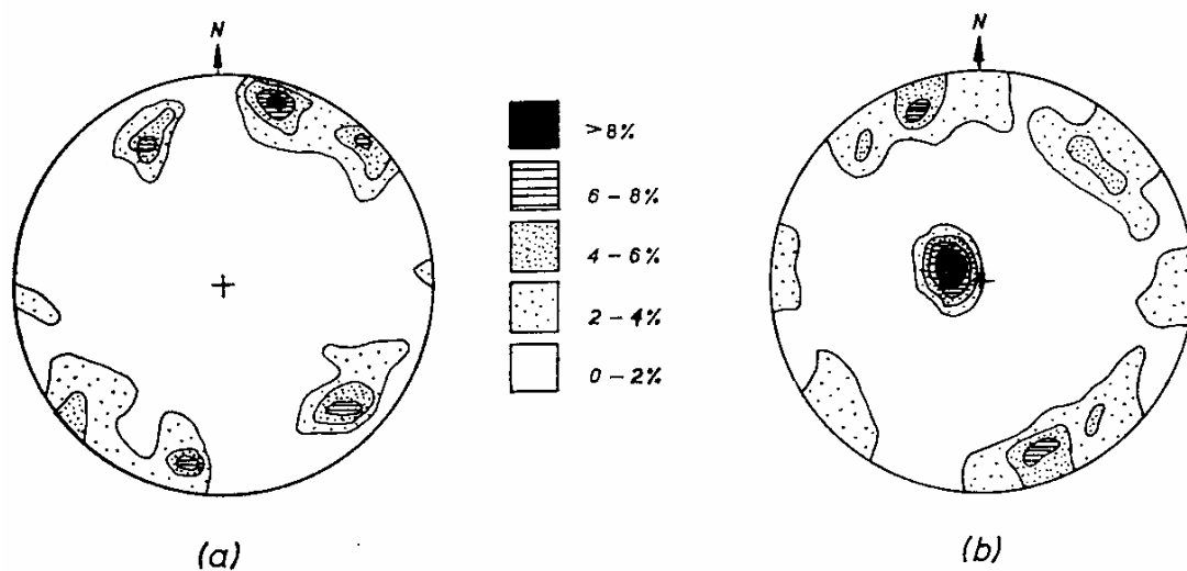
FIGURE 2. Stereographic plot of poles to planes for (a) joint planes in pelitic hornfelses and (b) pelitic hornfelses/granite contacts at Mousehole harbour.
