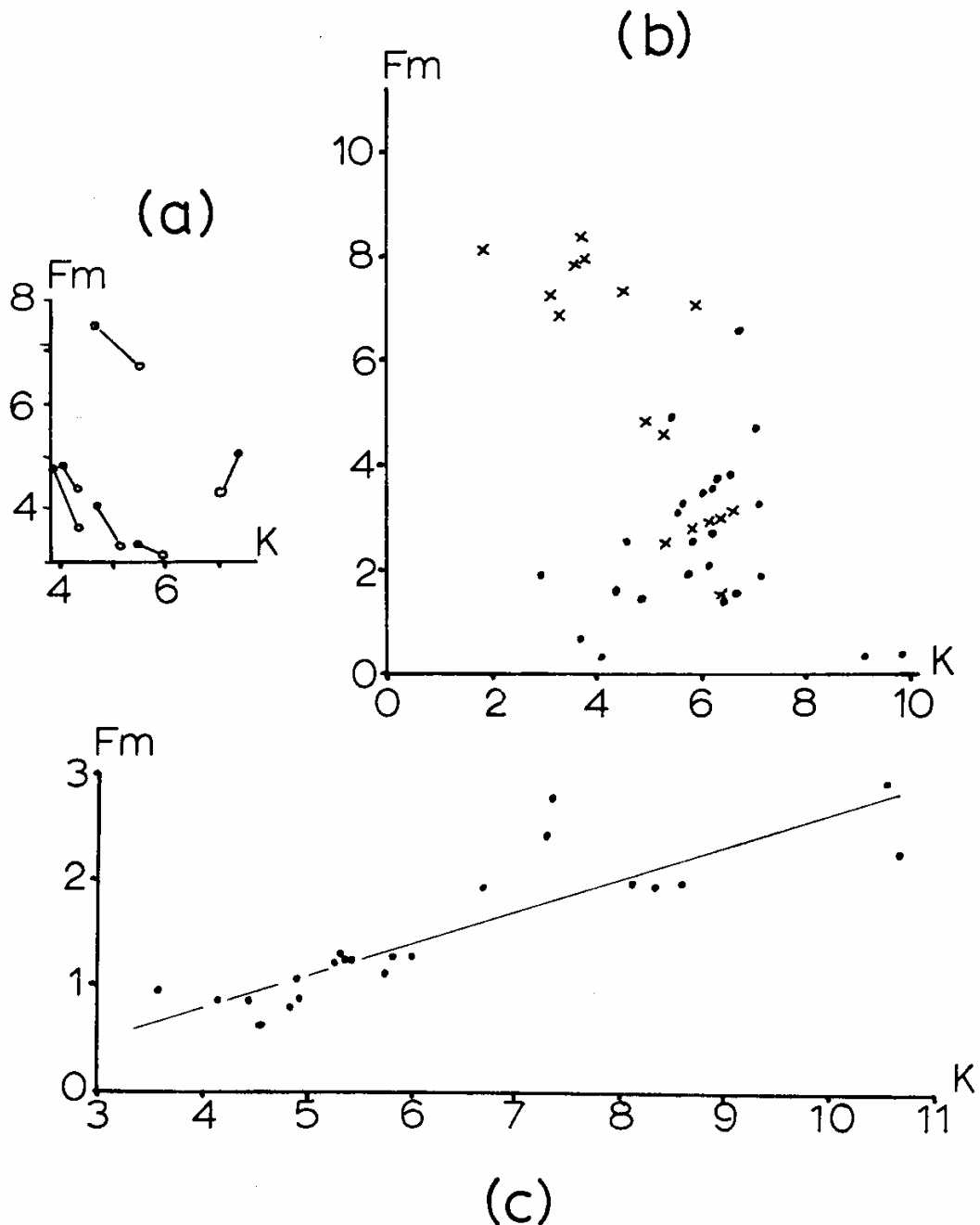
FIGURE 1. Fm-K variation diagrams (atomic percentages).
