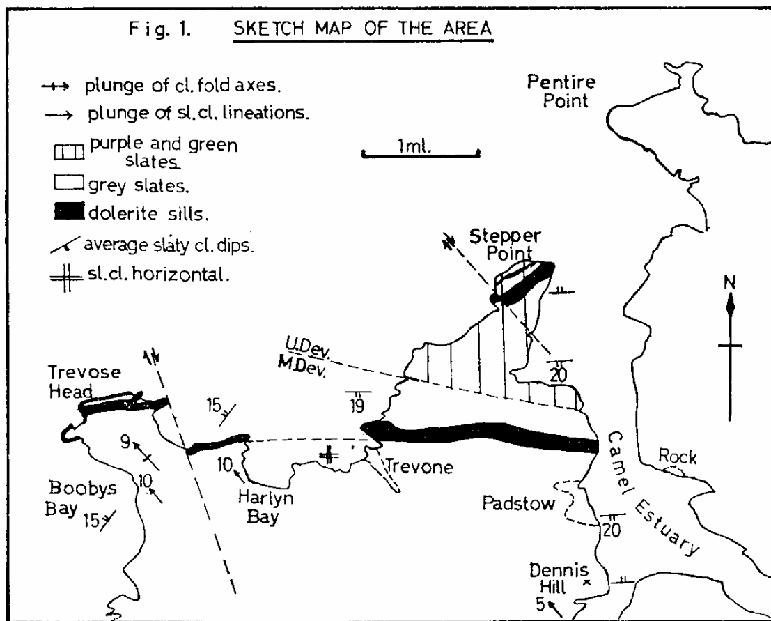
FIGURE 1. Geological sketch map showing regional variation in cleavage attitude and associated structures for the area west of the Camel Estuary.
