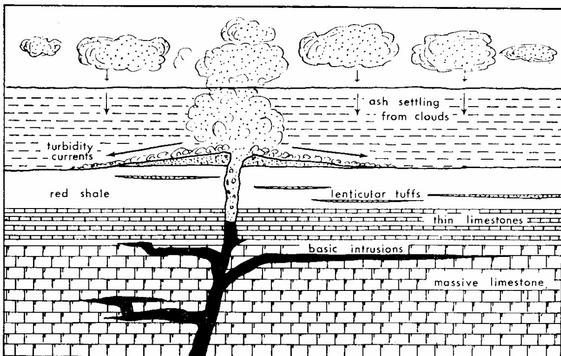
FIGURE 1. Hypothetical reconstruction of conditions of sedimentation in the Waterside Cove area during the Upper Devonian (Frasnian).
