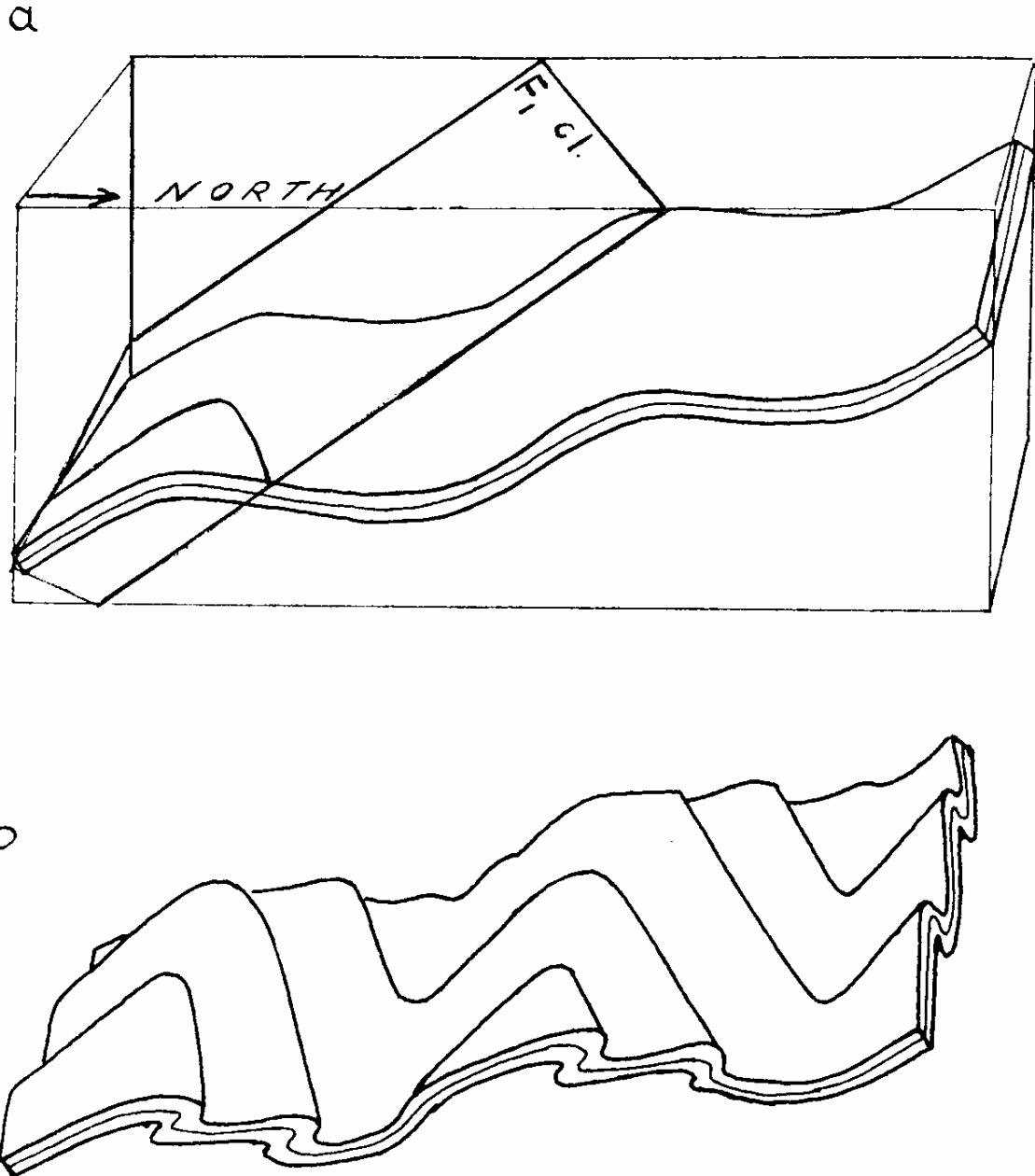
FIGURE 1. The relations between F_1 and postulated F_0 folds. (a) F_0 folds trending W.-E. (b) Superimposed F_1 folds.
