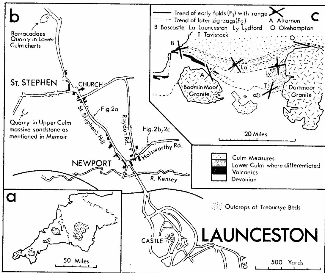
FIGURE 1. Location of the area in S.W. England. (a) Outline map. (b) Locality map for sections described. (c) Structural trends along south margin of the main Culm Measures outcrop.
