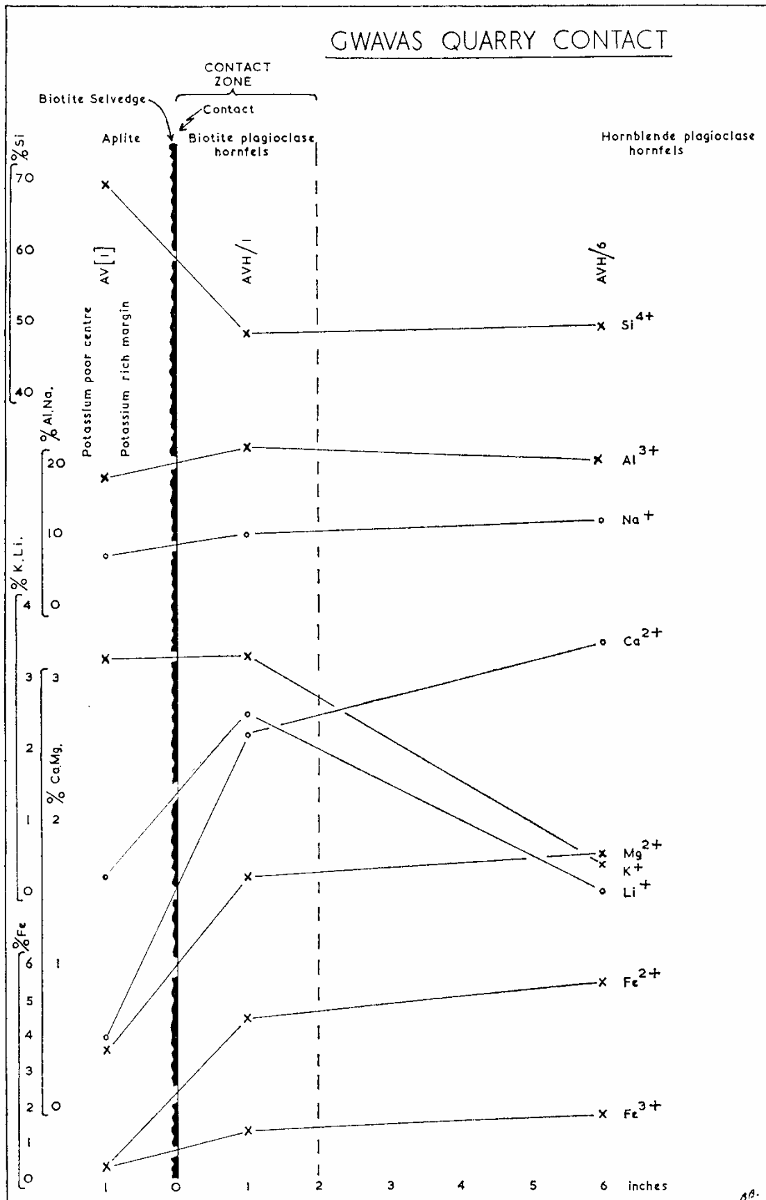
FIGURE 1. Cation per cent of various elements plotted against distance either side of the aplite/hornfels contact. The extent of the biotization is shown by the vertical dashed line between the biotite - plagioclase hornfels and the hornblende-plagioclase hornfels.
