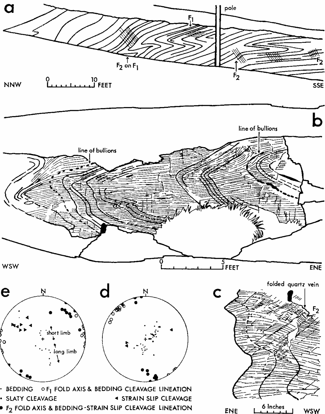
FIGURE 2. Structures in the Trebursye Beds of Launceston. (a) The St. Stephen's Hill section. Recumbent early folds ( F_1 ) with slaty cleavage crossed and deformed by second folds ( F_2 ) with strain slip cleavage. (b) New section in Holsworthy Road with first folds ( F_1 ) and slaty cleavage. (c) New section in Holsworthy Road showing coarse strain-slips cutting and bending ( F_2 ) slaty cleavage in early folds. (d) Stereogram (lower hemisphere) of structures in the Newport exposures. (e) Stereogram of St. Stephen exposures.
