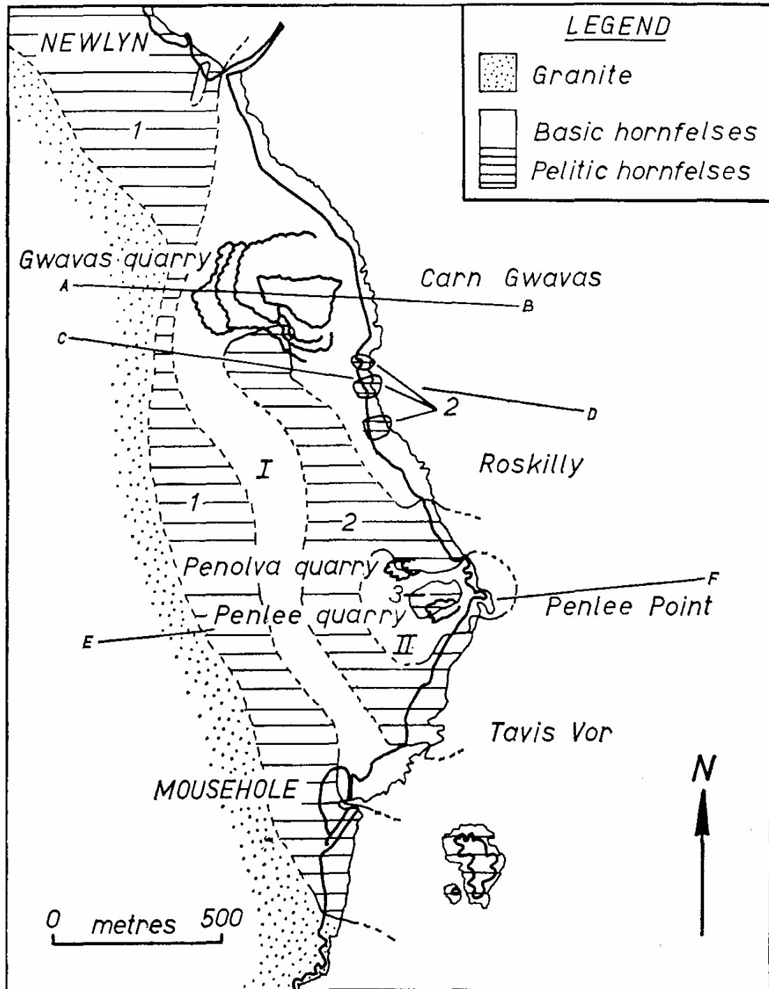
FIGURE 1. Geological map of the Land's End aureole between Mousehole and Newlyn, Cornwall, showing the Gwavas sill (I) and the Penlee sill (II). All rocks have an eastward dip.
