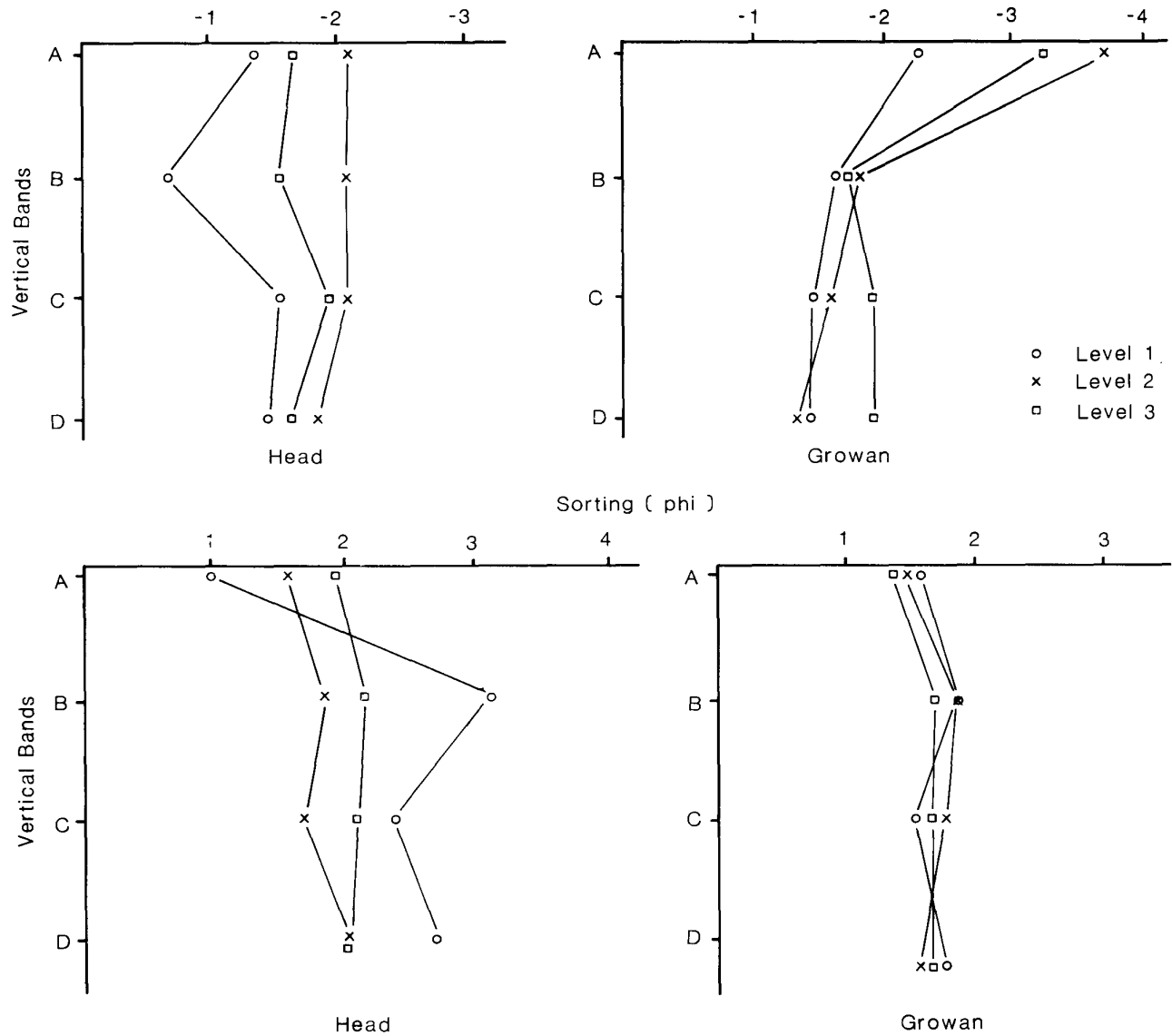
Figure 6. Lateral variation in median grain size and sorting coefficients for the Dunnabridge exposure.
