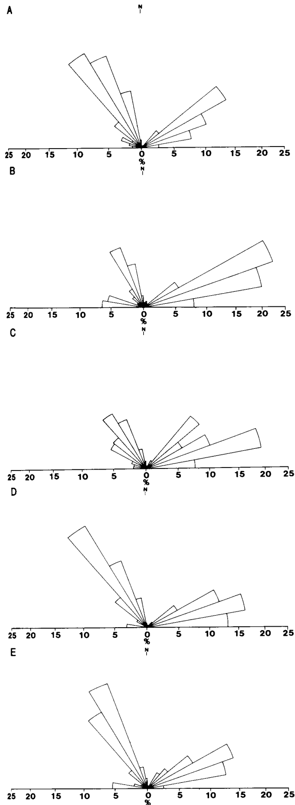
Figure 6. Percentage weighted rose diagrams for each area (percentage of lineaments within 10^\circ arc). The total numbers of lineaments are given for each area below: A South West England (311) B South Devon (266) C South Cornwall (260) D North Devon (363) E Bodmin (241)
