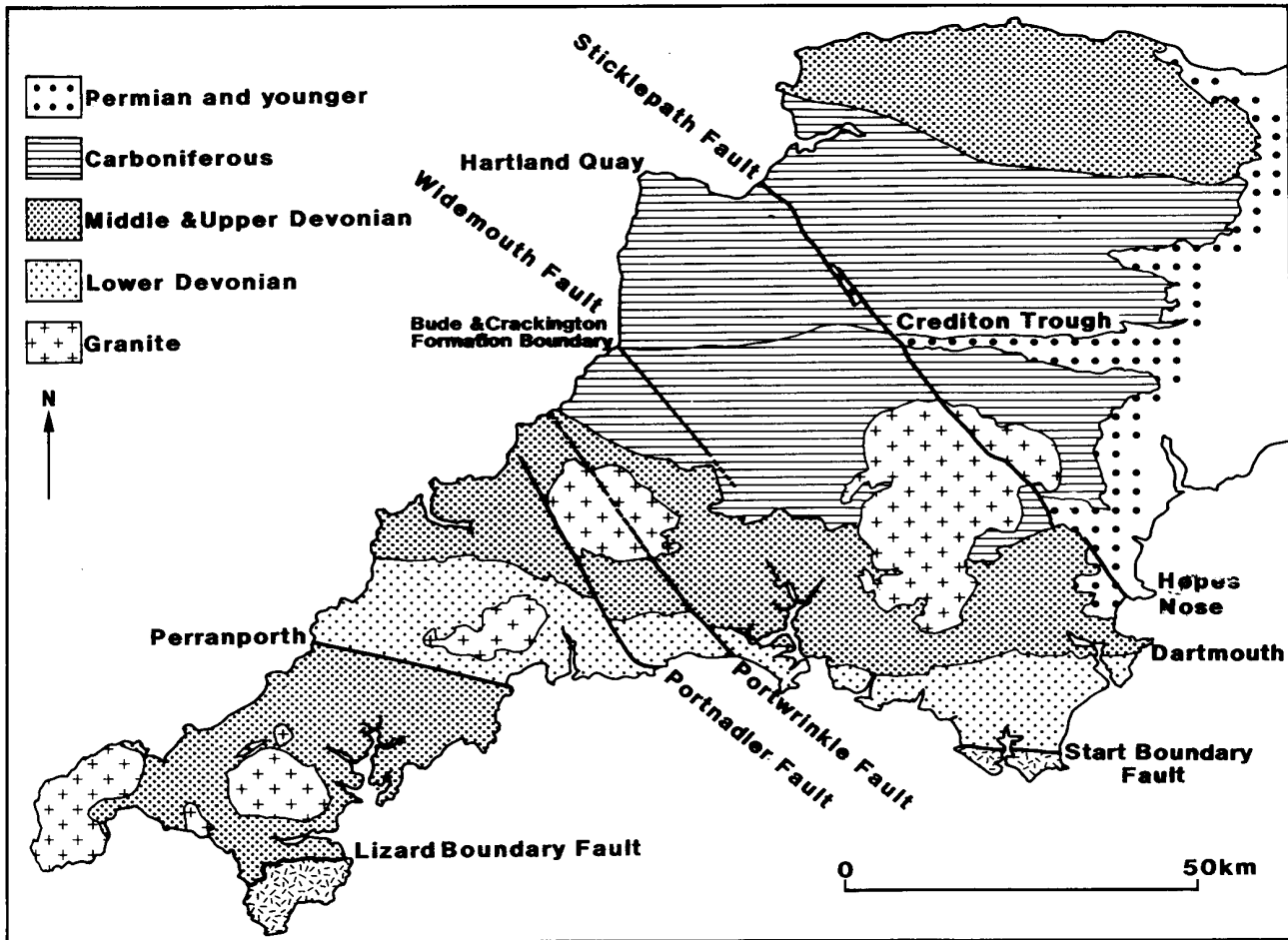
Figure 1. Simplified geological sketch map of South West England.
