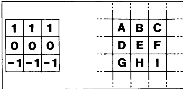
Figure 2. The DN (A etc) for each pixel is overlain by the convolution matrix and is multiplied by the corresponding weighting factor - Ax1 , Bx1 , Cx1 etc. The products are then summed to compute the value to be used in place of the DN of the pixel beneath the centre of the convolution matrix. E. The operation is performed on all the pixels in the image.
