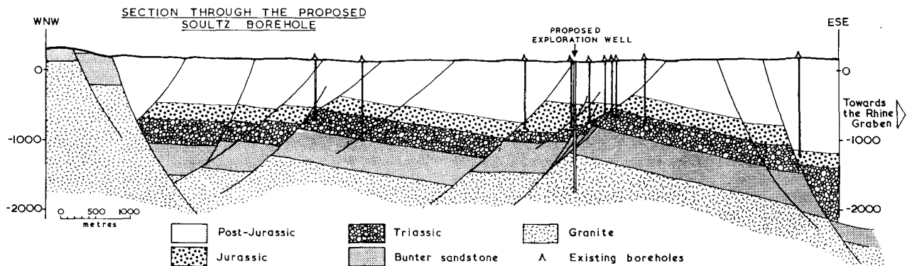
Figure 5. Simplified cross-section of the Rhine Valley through the Soutz site.
